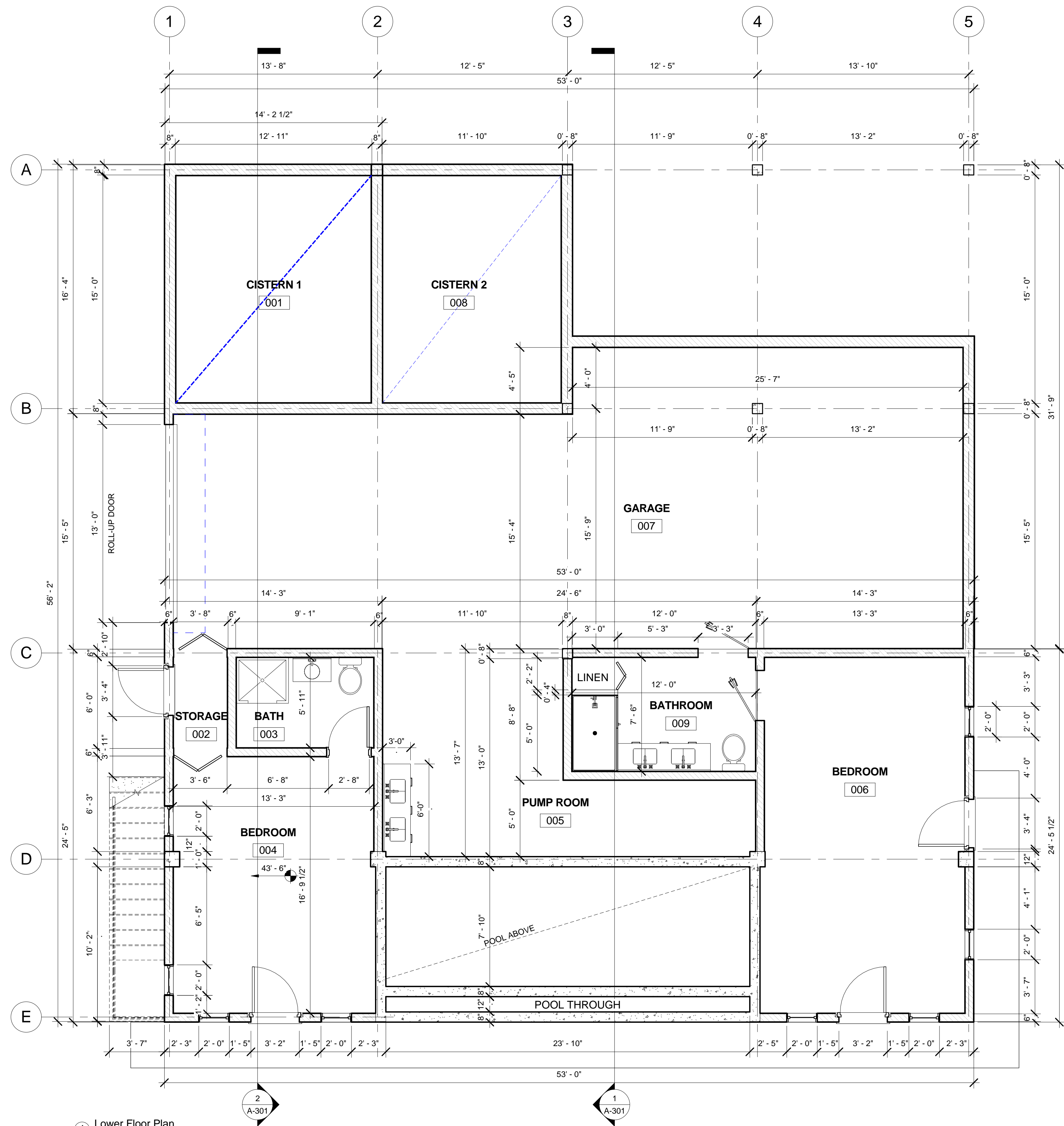
1 Lower Floor Plan 1/4" = 1'-0"
